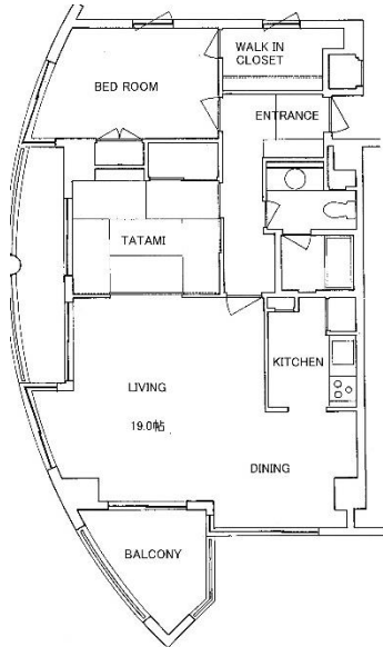
Atype 107,207,307,407 83.14m 2
