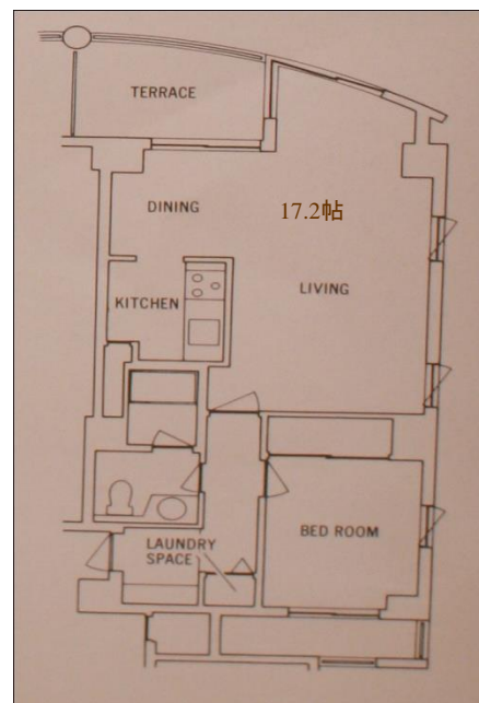
Ftype 201,301,401,501 60.72㎡
